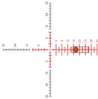
17.5 MOA reticle holdover at 625 yards. No wind. Illustration shown is the 2-10 x 32.
